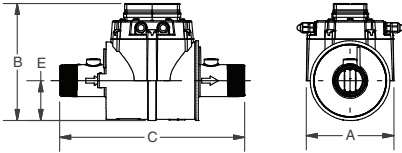
NPT / BSP WITH 09 ELECTRONICS
